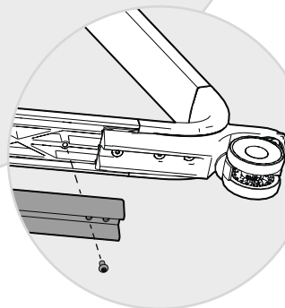
Board Pro 55
